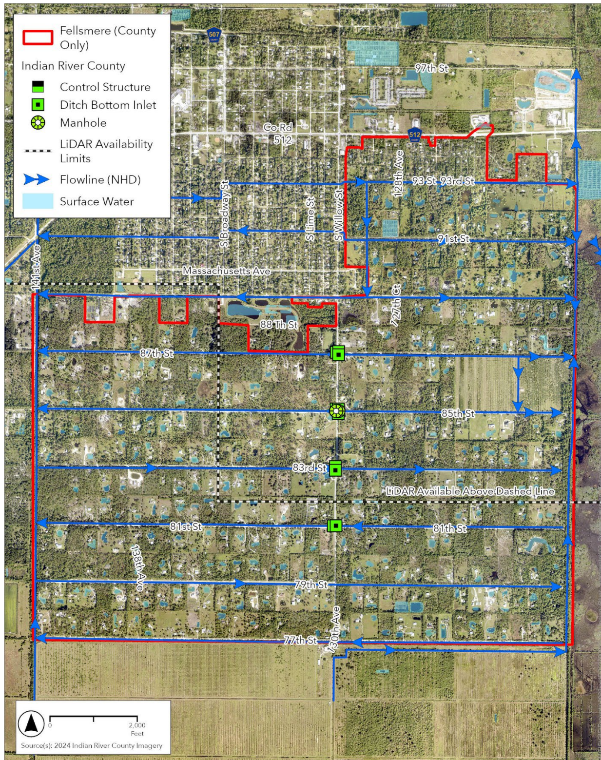
Figure 45 Stormwater Features within Fellsmere Priority Area
