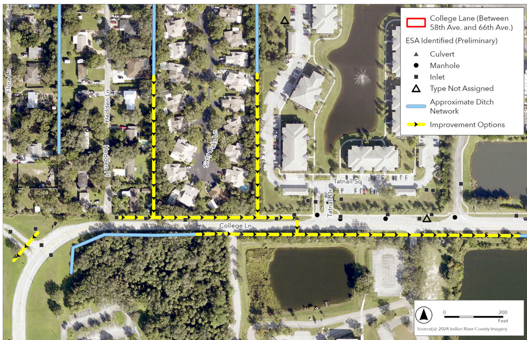
Figure 37 College Lane Proposed Conceptual Improvement Option #1
