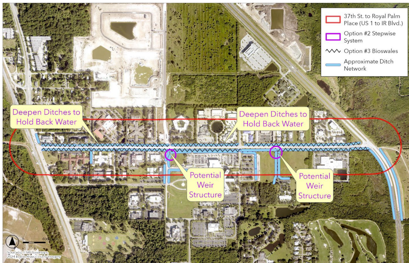
Figure 43 Proposed Conceptual Improvement Option #2 and Option #3 for 37 th Street
