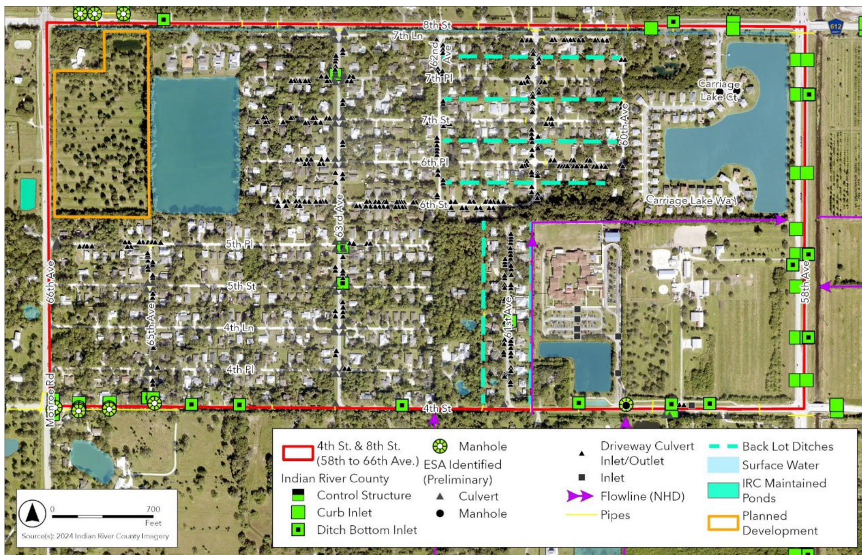
Figure 50 Stormwater Features within 4 th and 8 th Priority Area
