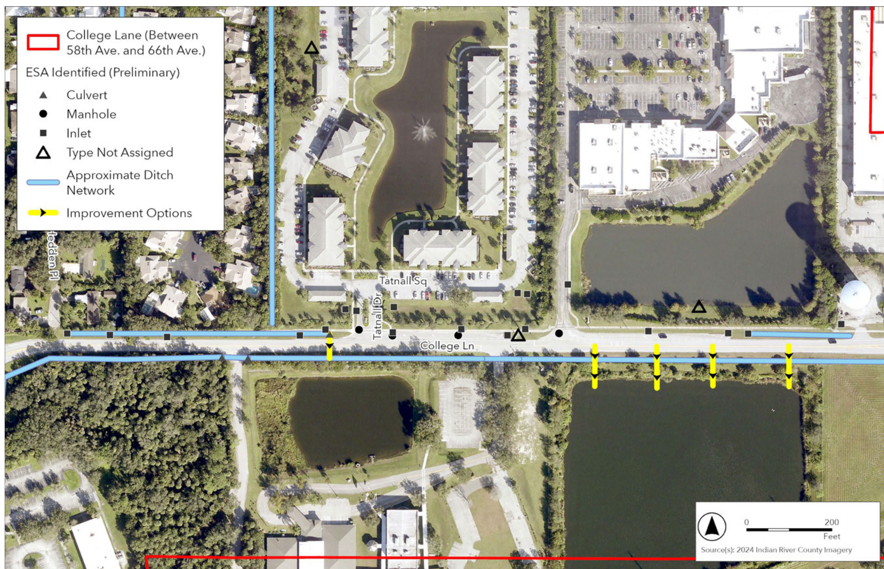
Figure 38 College Lane Proposed Conceptual Improvement Option #2
