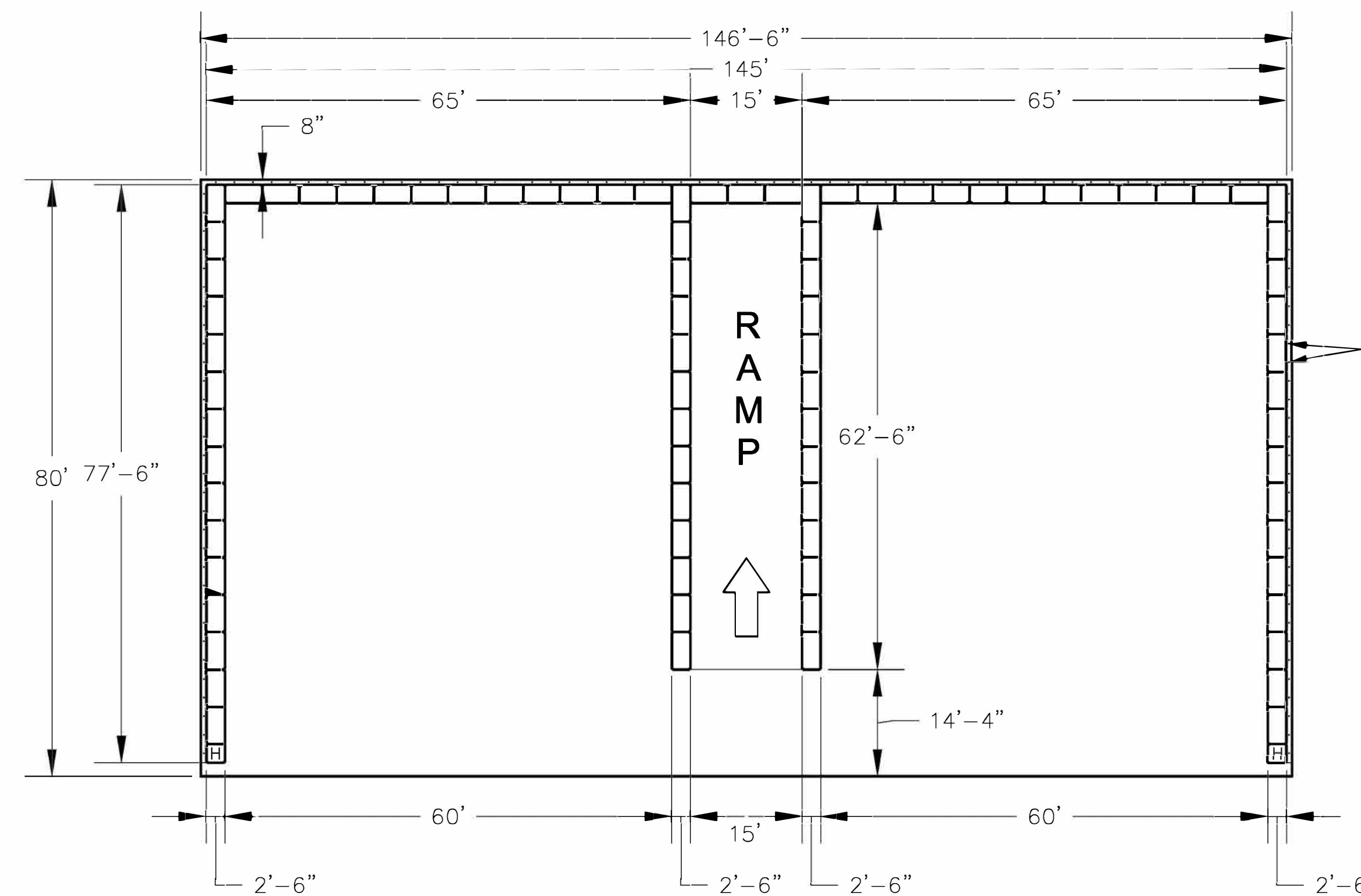
PLAN VIEW - 1st Course
