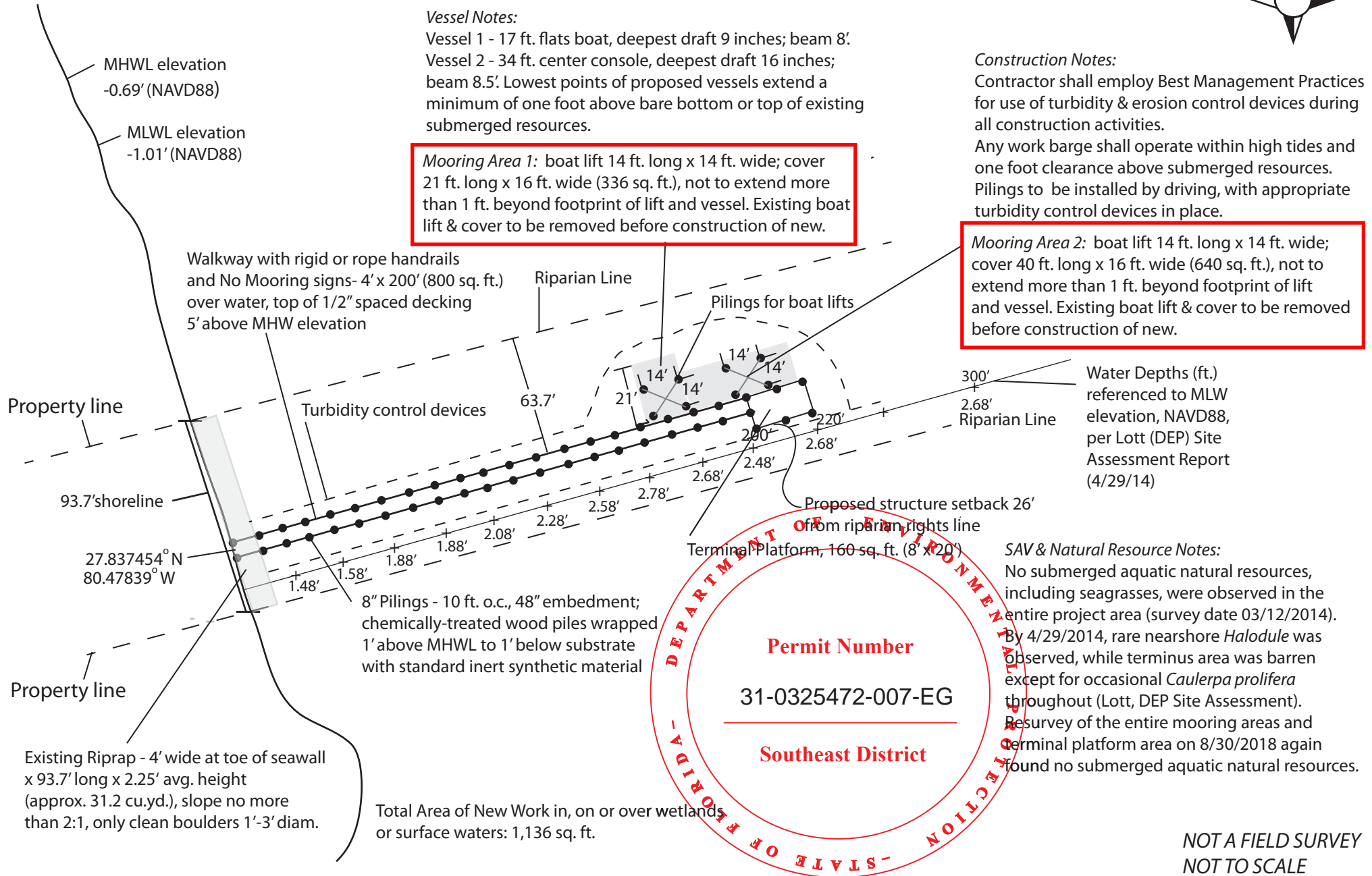
Figure 3: Plan View
